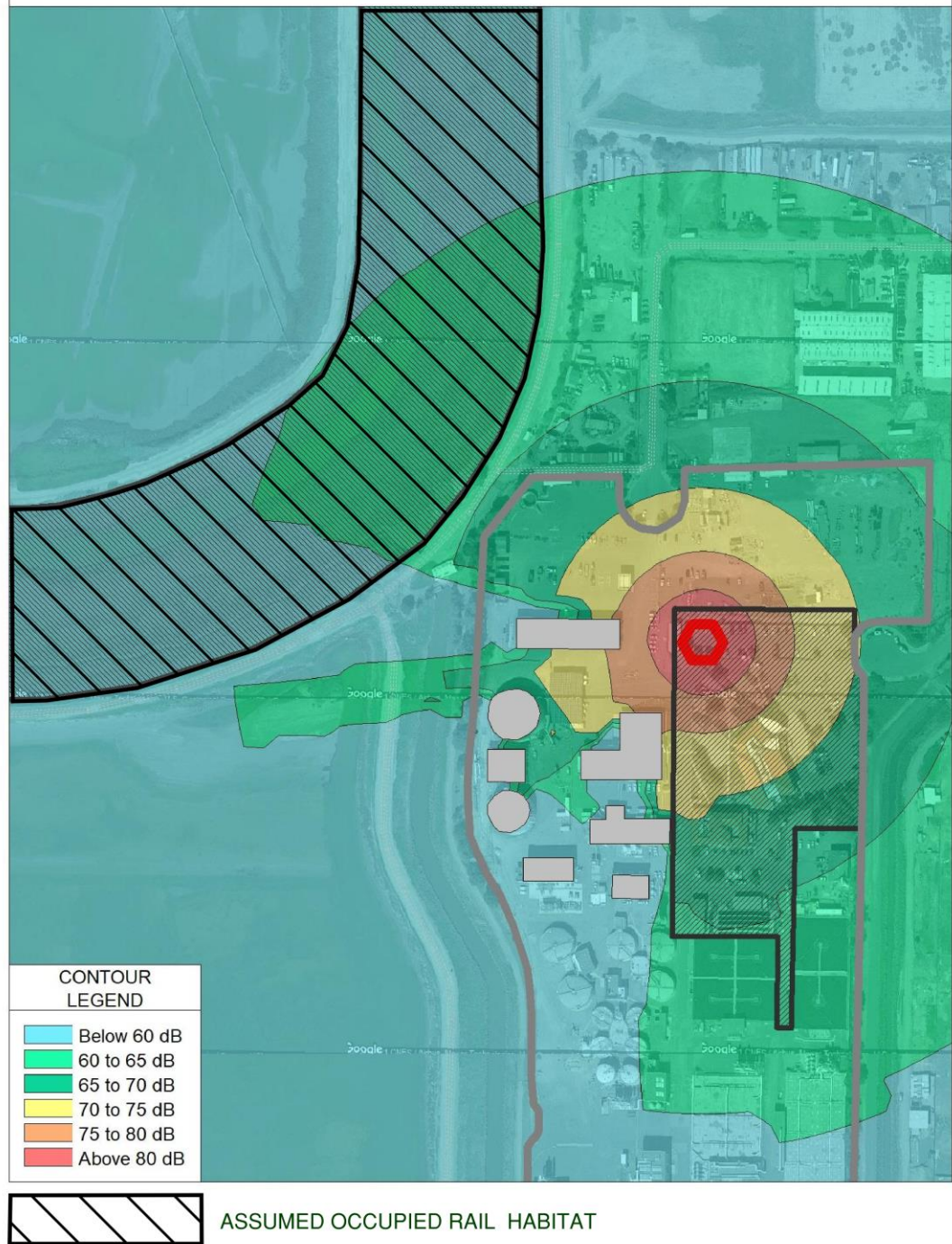
Union Sanitary District Phase 1B Estimated Construction Noise Contour Map Figure 4: One Construction Source (generating 85 dBA at 50')
