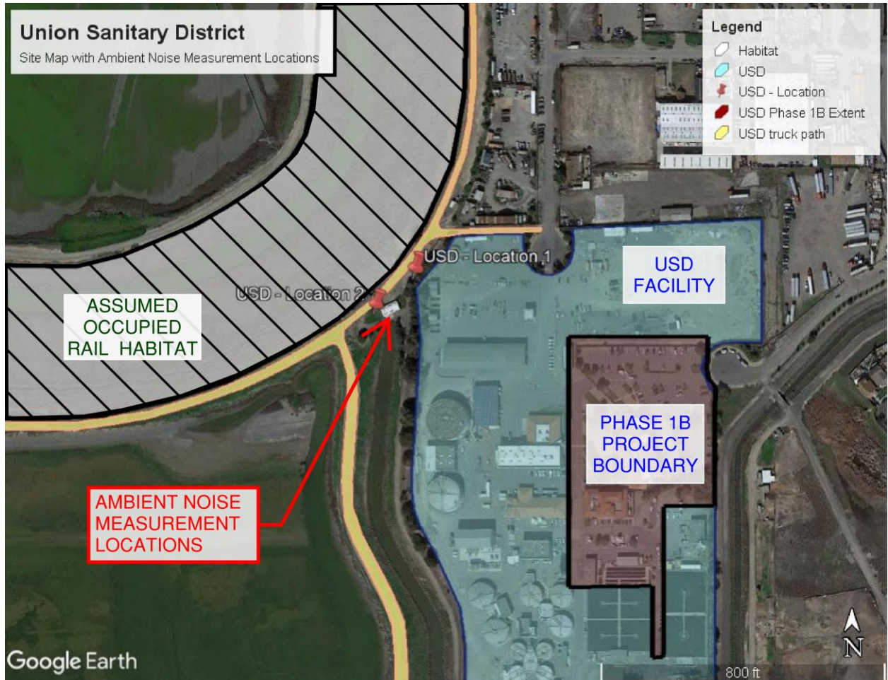
Figure 2: Site plan identifying ambient noise measurement locations
