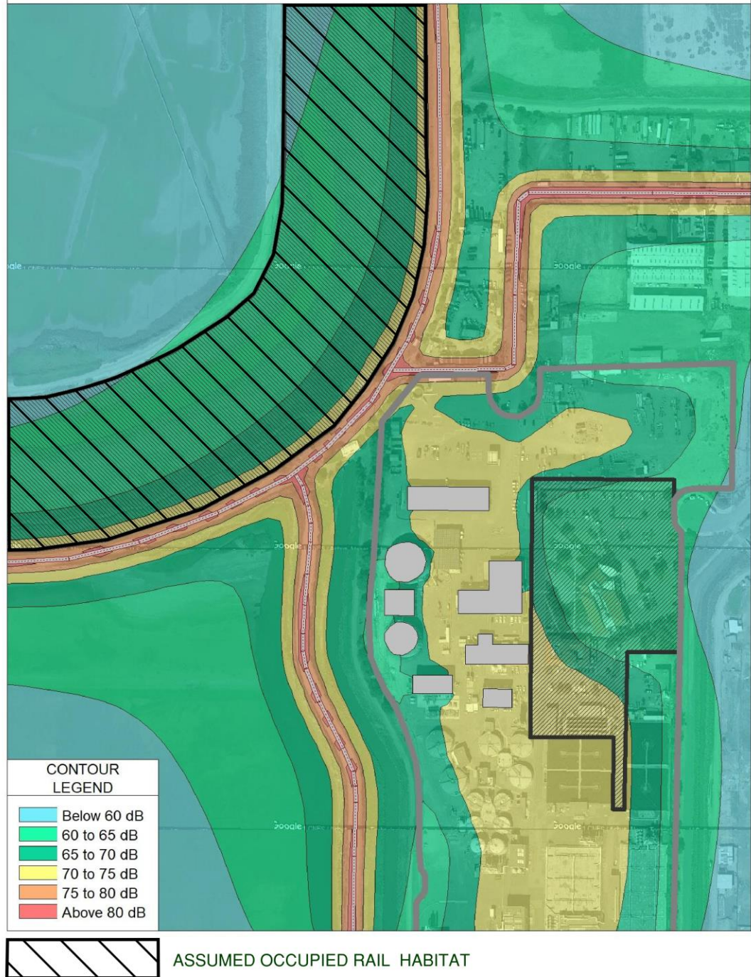
Union Sanitary District Phase 1B Estimated Construction Noise Contour Map Figure 3: Maximum Ambient Levels from Trucks and USD Operations
